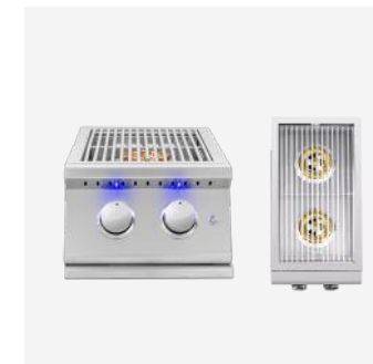
SIZZLER PRO LIGHTED DOUBLE SIDE BURNER SIZPROSB2 • Total BTUs: 24,000 • Cooking Surface: 19½ x 10¼ • Front Panel LED Lighting
