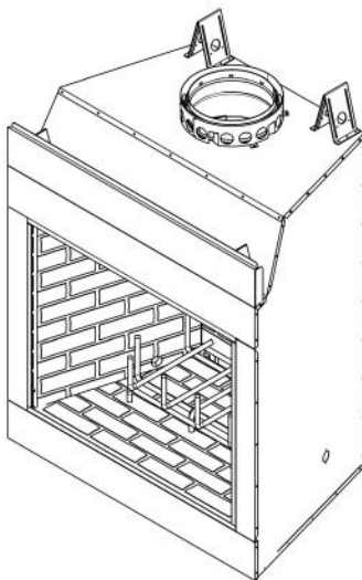
WOODBURNING FIREPLACE
