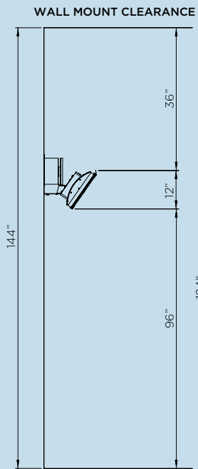
WALL MOUNT CLEARANCE + HEAT DEFLECTOR
